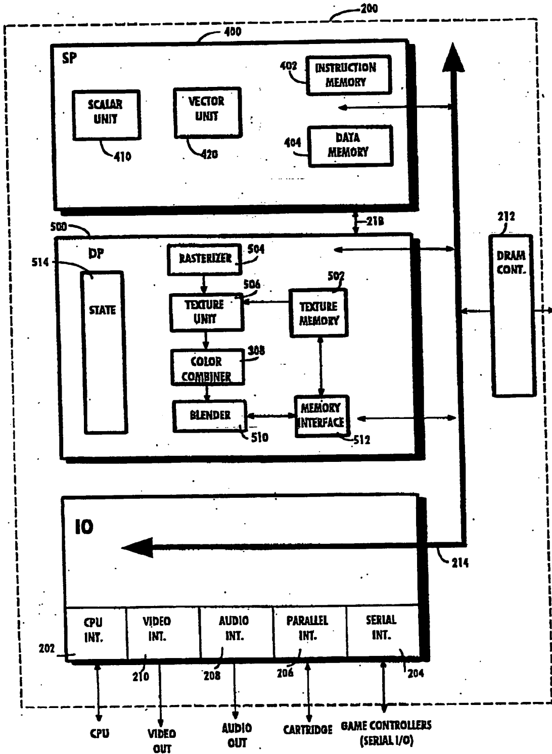
Fig. 6 COPROCESSOR
